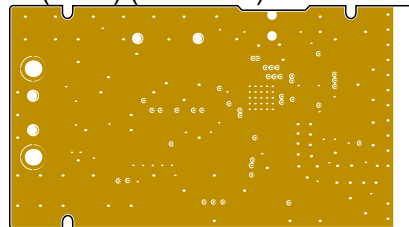
L2(GND) (Scale 1:1)
