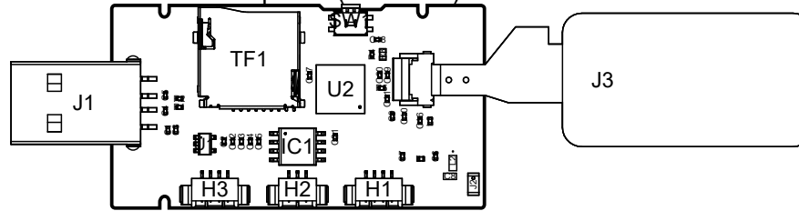
View from Bottom side (Scale 1:1)
